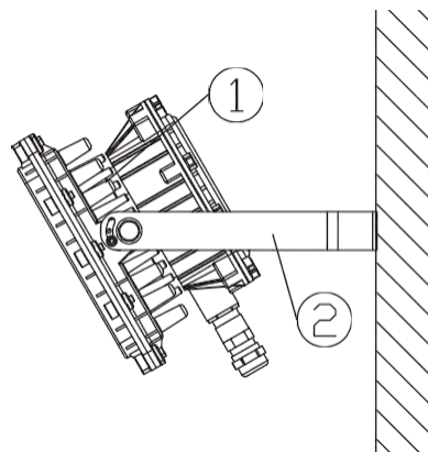
Wall type
